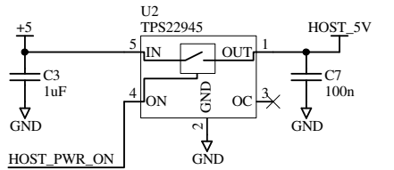
USB 5V Supply: 100mA Current limited switch
